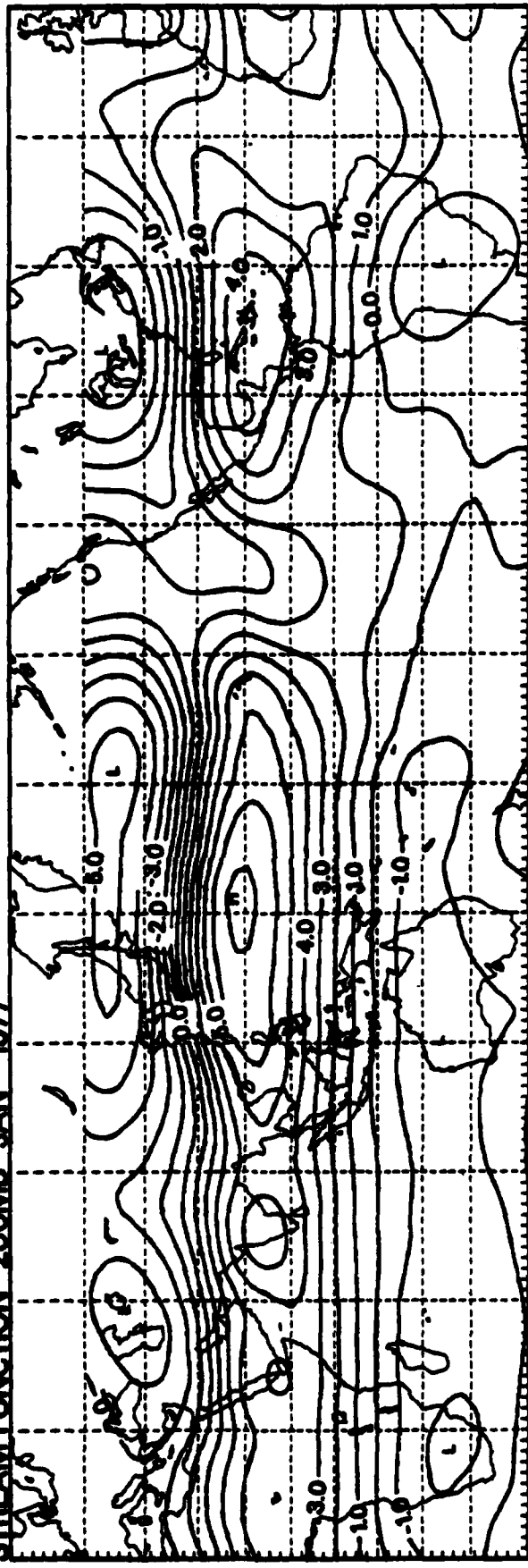
STREAM FUNCTION 200MB JAN 1977
